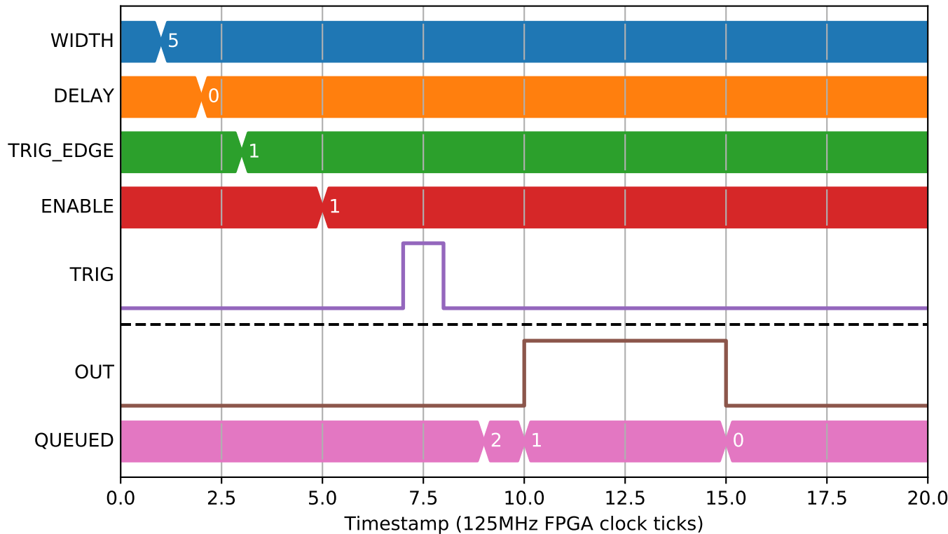
Pulse stretching with no delay activate on falling edge
