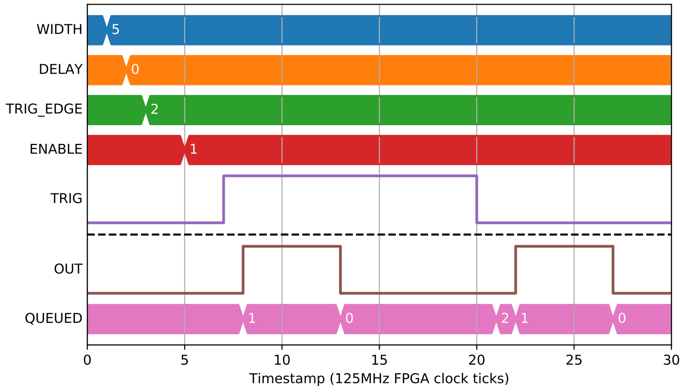
Pulse stretching with no delay activate on both edges
